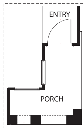
ELEV. 'B' FRONT PORCH
