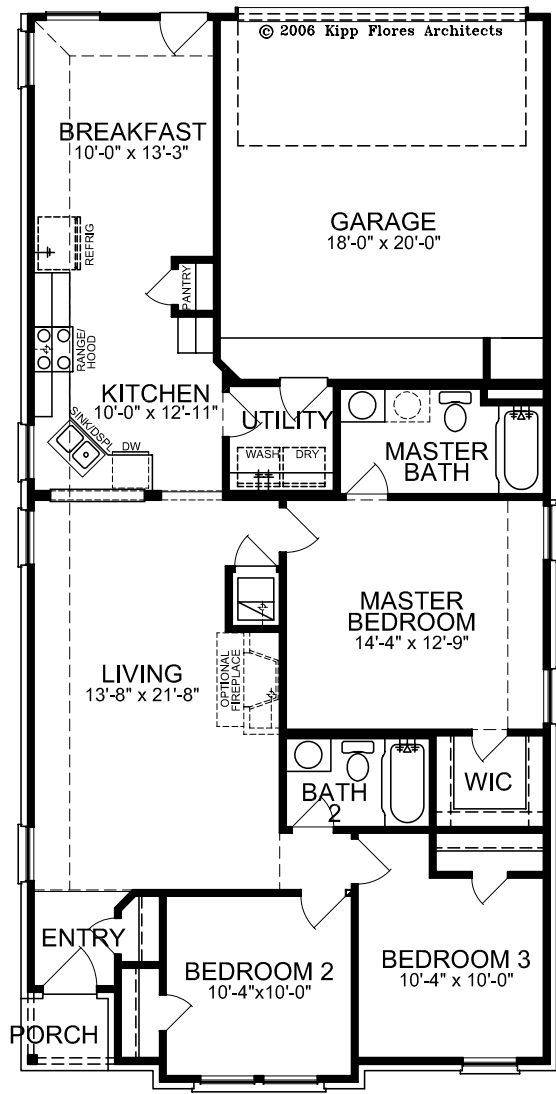
FLOOR PLAN 1357
